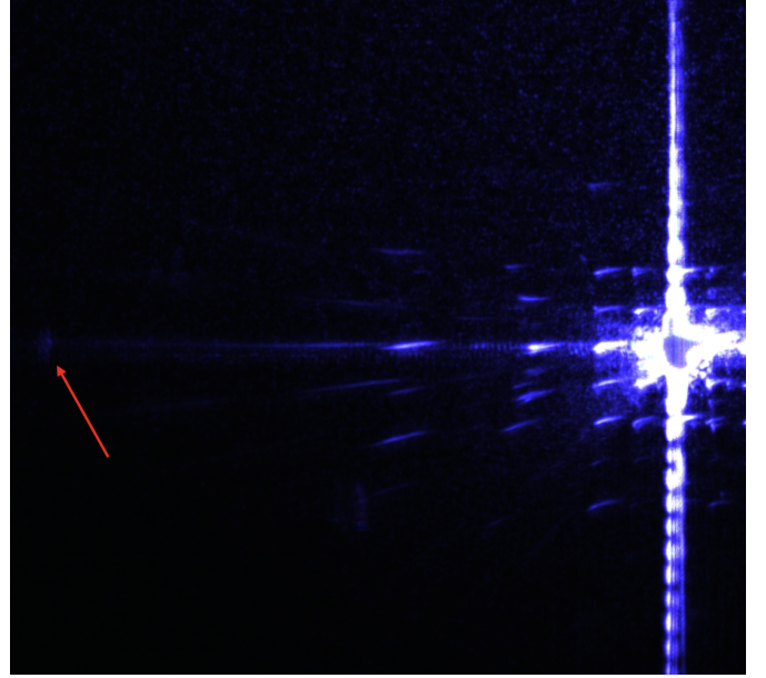
(a) Digits 1 vs. 1. After reducing the range to only capture the left part of the correlation plane, a (hard to see) off-axis peak (red arrow) reveals the high similarity of the two inputs.
